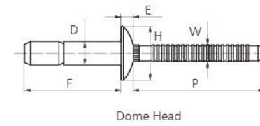
Dome Head
