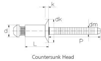
Countersunk Head
