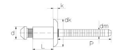
Large Flange
