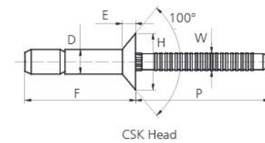
CSK Head
